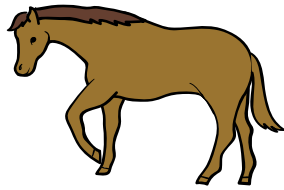
horse
