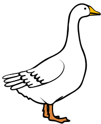
goose
