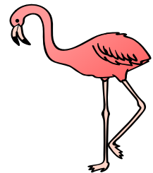
flamingo
