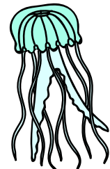
jellyfish
