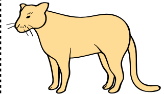
puma
